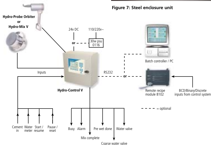
Figure 8: System interfacing schematic
