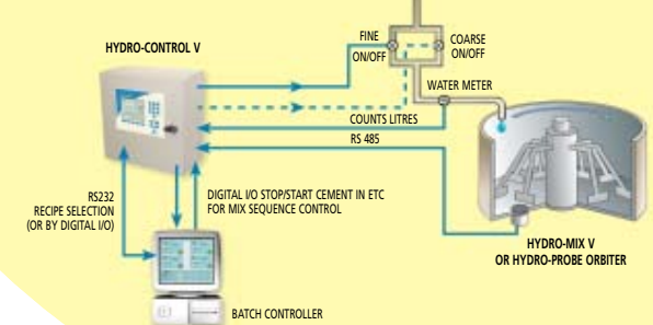
Figure 6: System overview integrated with batch control system
