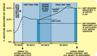
Figure 2: Typical mix cycle – Calculation mode
