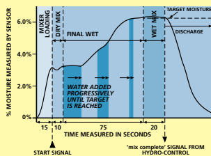
Figure 1: Typical mix cycle – Auto mode
