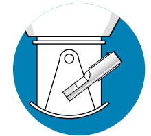
Scheme 3 Hydro-Probe II may be inclined down at approx 45° to minimise obstruction to the flow, when neck of bin is small.
