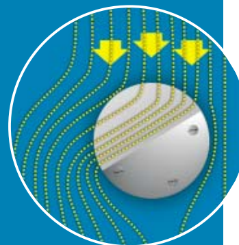
Scheme 7 Where space is very restricted, the Hydro-Probe II may be positioned below the bin to avoid flow obstruction
